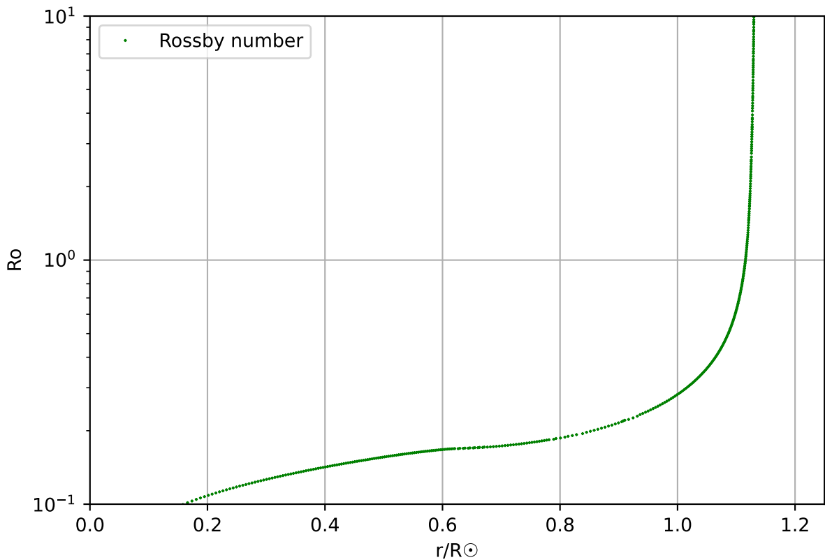
Rossby number, profile 105, age 1.43 \times 10^7
